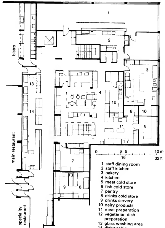
⑪ Kitchen for 100 standard meals, 100 speciality meals, 120 bistro covers and 80 staff meals
